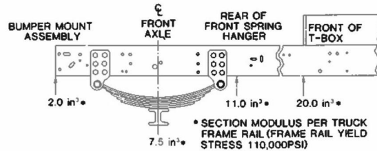
Standard Truck Frame—for angled single front stabilizer only
