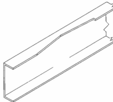
Extended Truck Frame—for angled or straight down single front stabilizer
